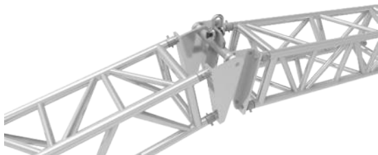
Ceiling Support It is flexible hanging point which reduce the problem of 100% simultaneous lifting
